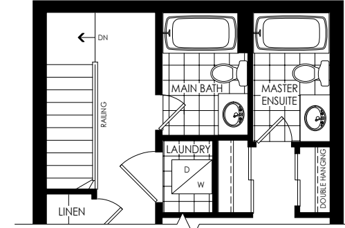
ELEVATION AB, AC, BB, BC FLEX PLAN WITH LAUNDRY
